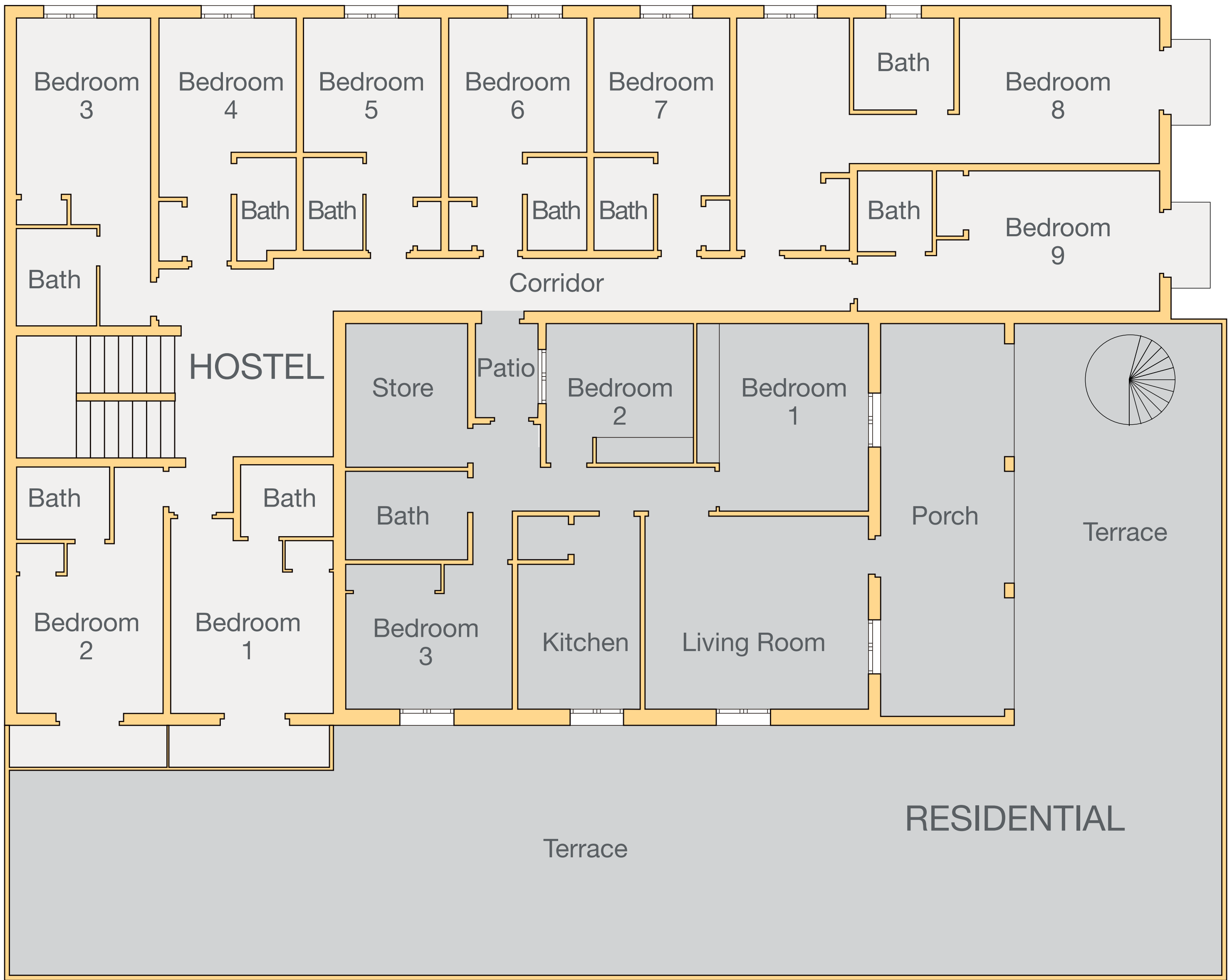
First Floor
